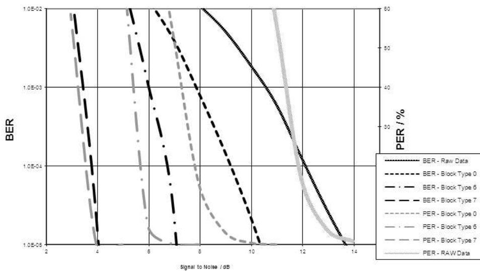
Figure 43 Comparison of BER and PER for 4-QAM Modulation
