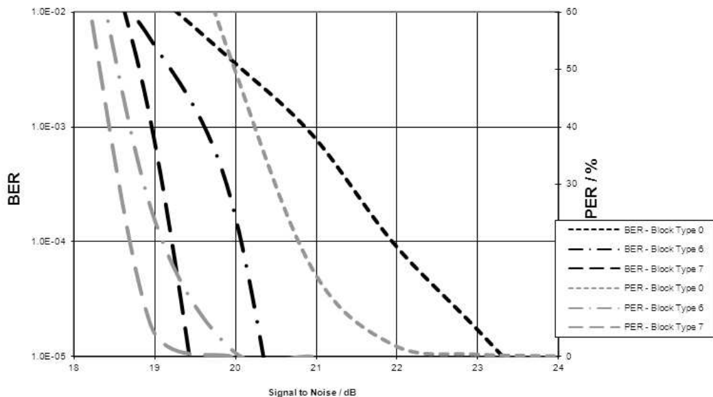
Figure 45 Comparison of BER and PER for 64-QAM Modulation
