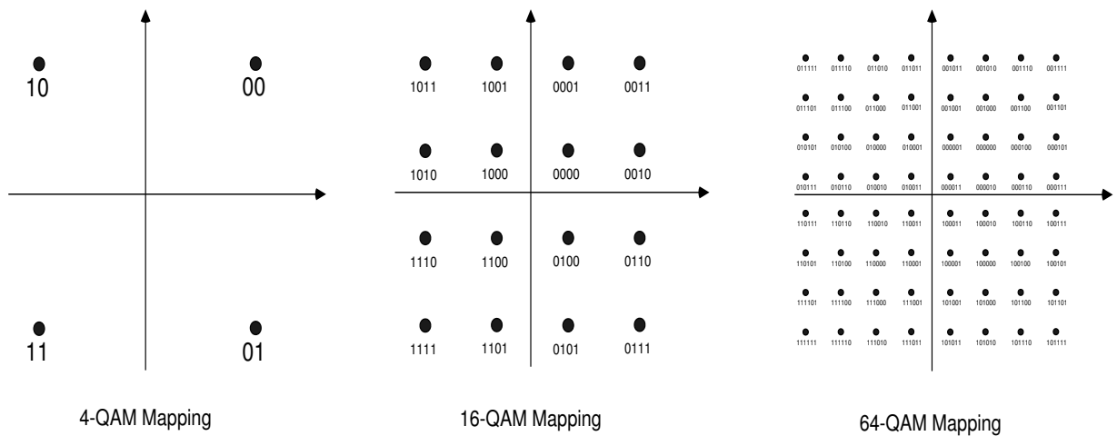
Figure 28 QAM Mappings
