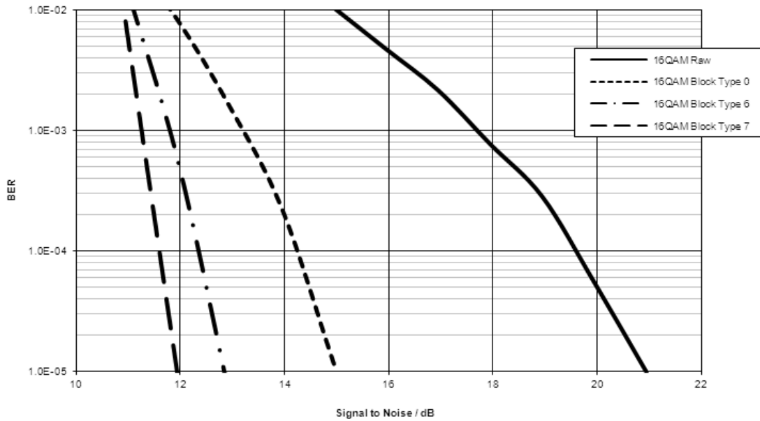
Figure 41 16-QAM Performance with Different Coding Schemes
