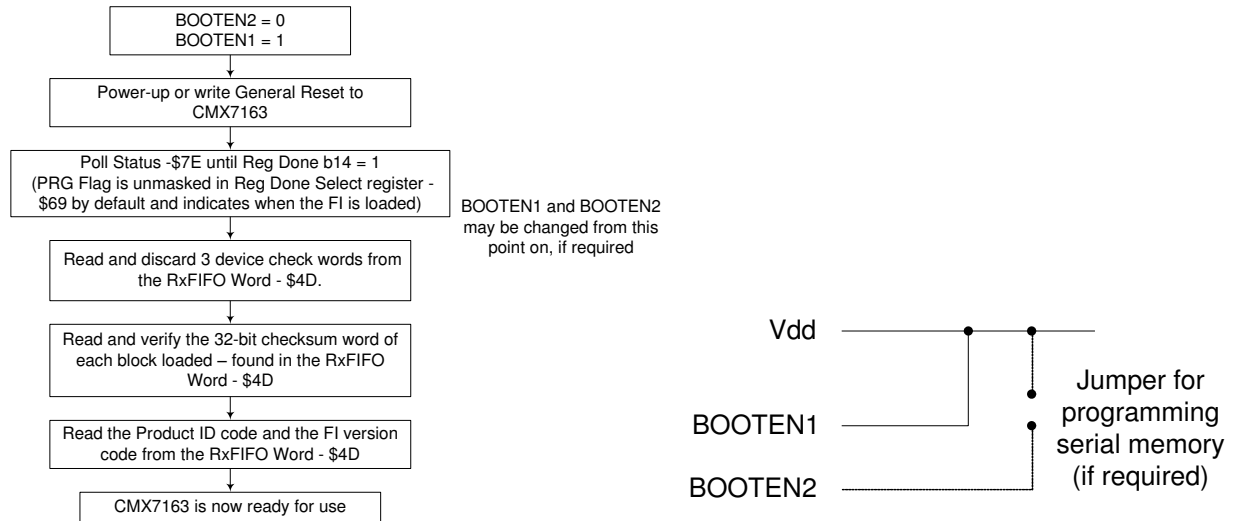
Figure 9 FI Loading from Serial Memory
