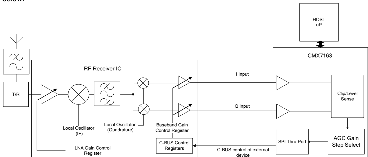
Figure 24 AGC using SPI Thru-Port
