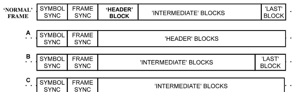
Figure 30 Suggested Frame Structures
