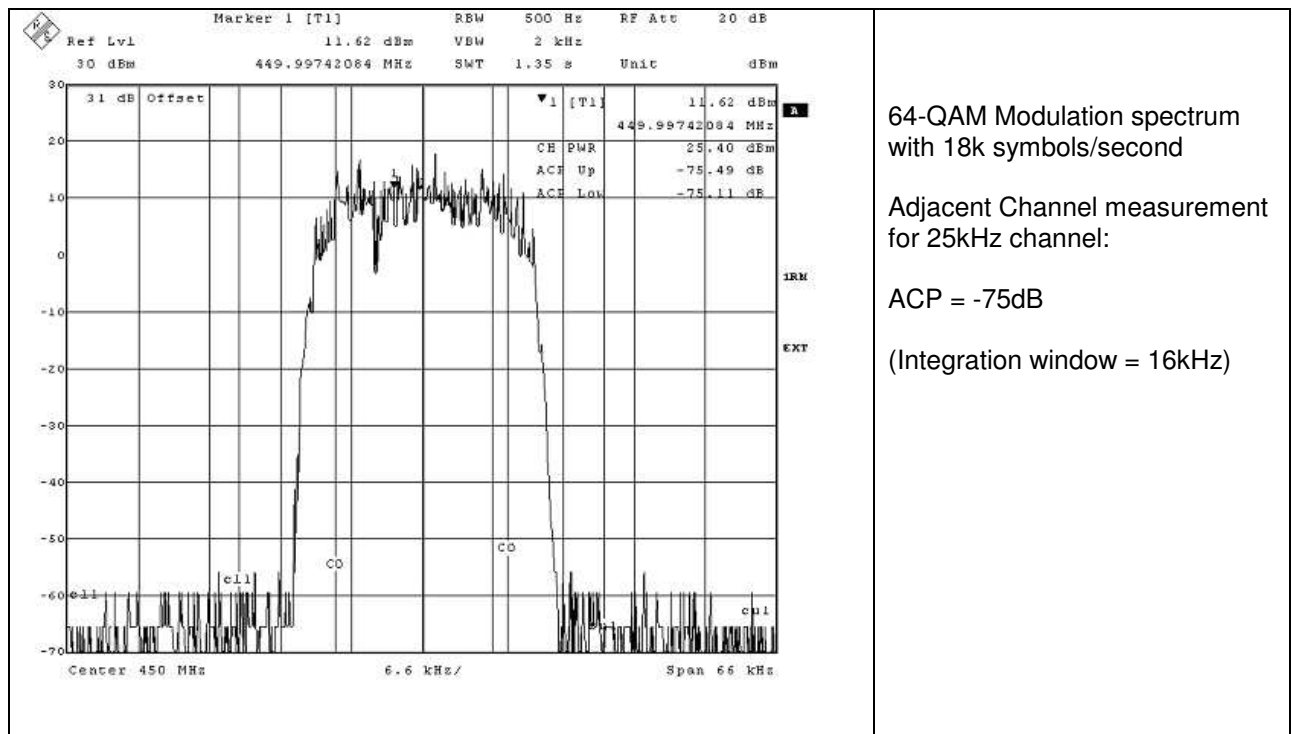
Figure 36 Tx Modulation Spectra (64-QAM), 18ksymbols/sec I/Q Modulation into CMX998
