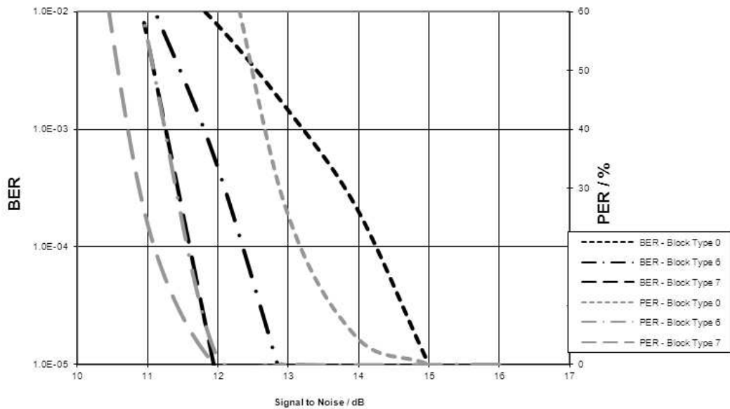
Figure 44 Comparison of BER and PER for 16-QAM Modulation
