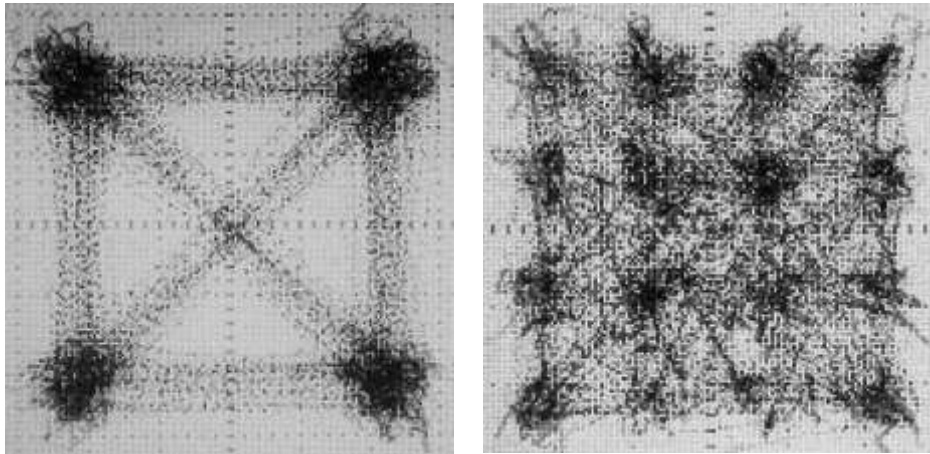
Figure 31 Received 4 and 16-QAM signals, no equalisation
