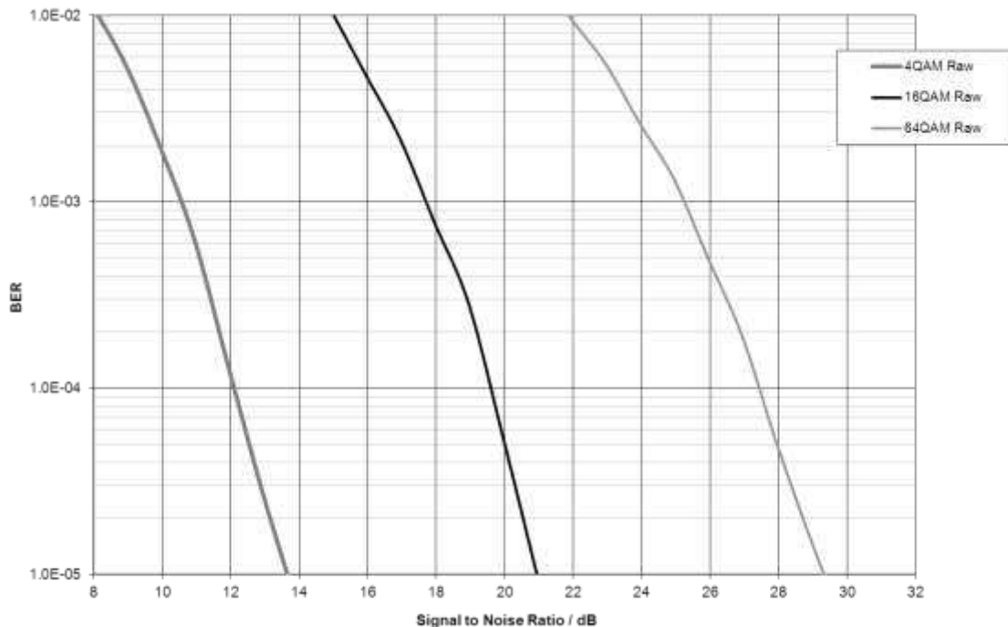
Figure 38 Modem Sensitivity Performance
