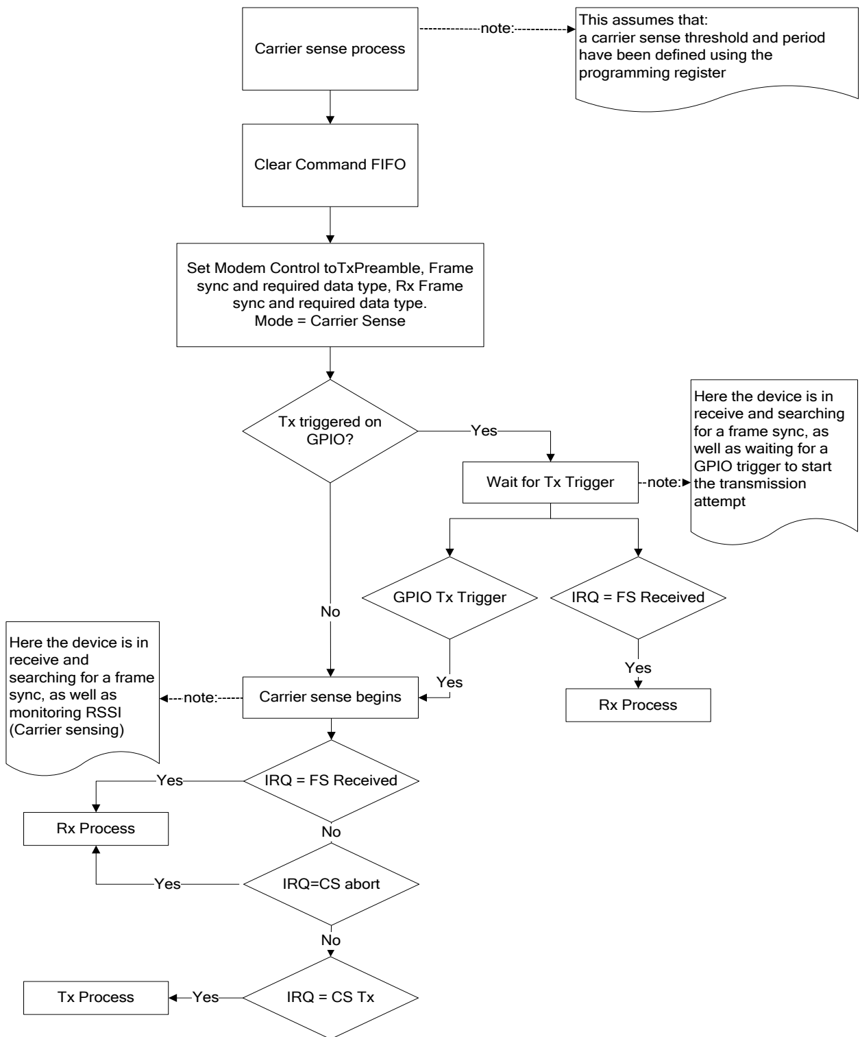
Figure 12 Carrier Sense
