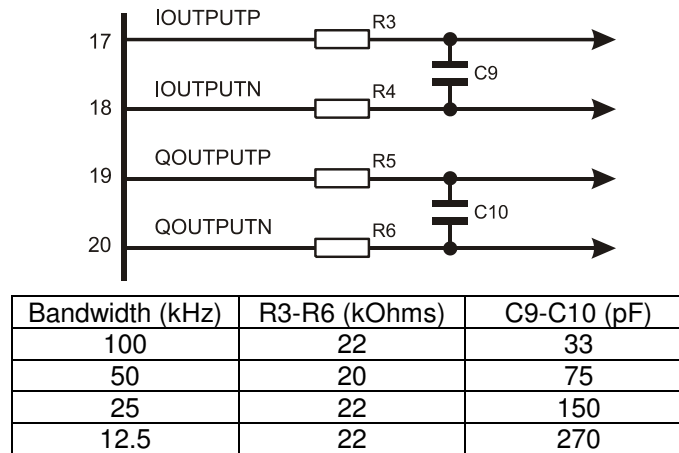
Figure 6 Recommended External Components – I/Q Output Reconstruction Filter
