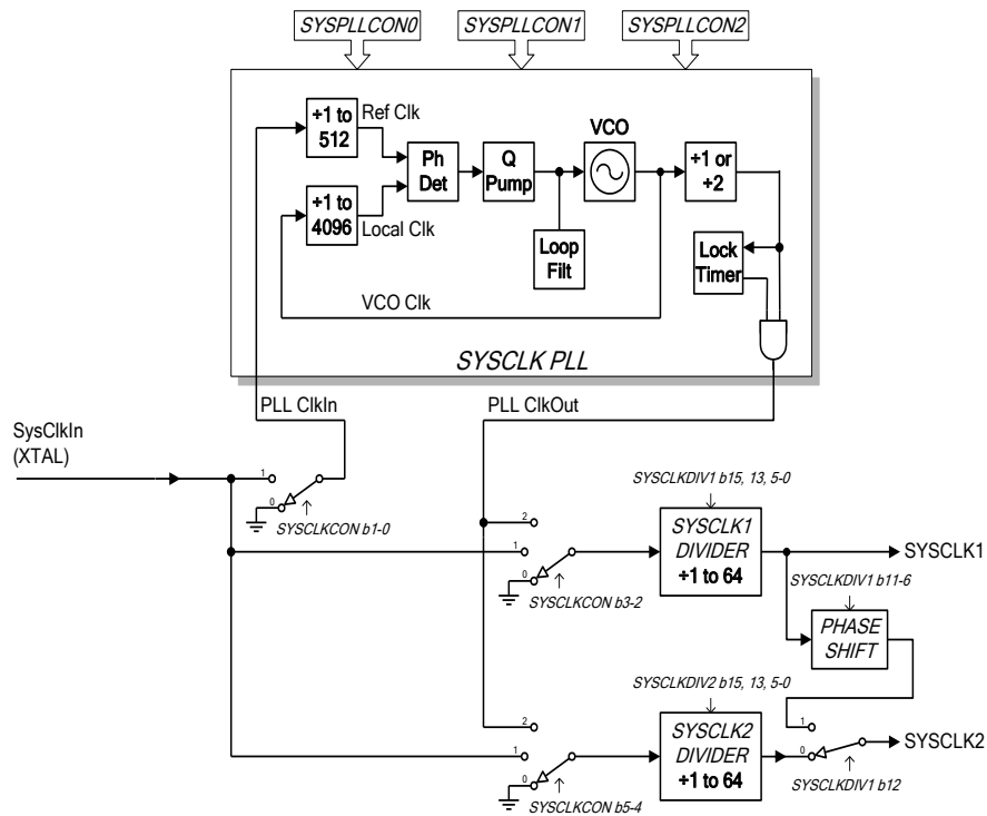
Figure 27 Digital System Clock Generation Schemes
