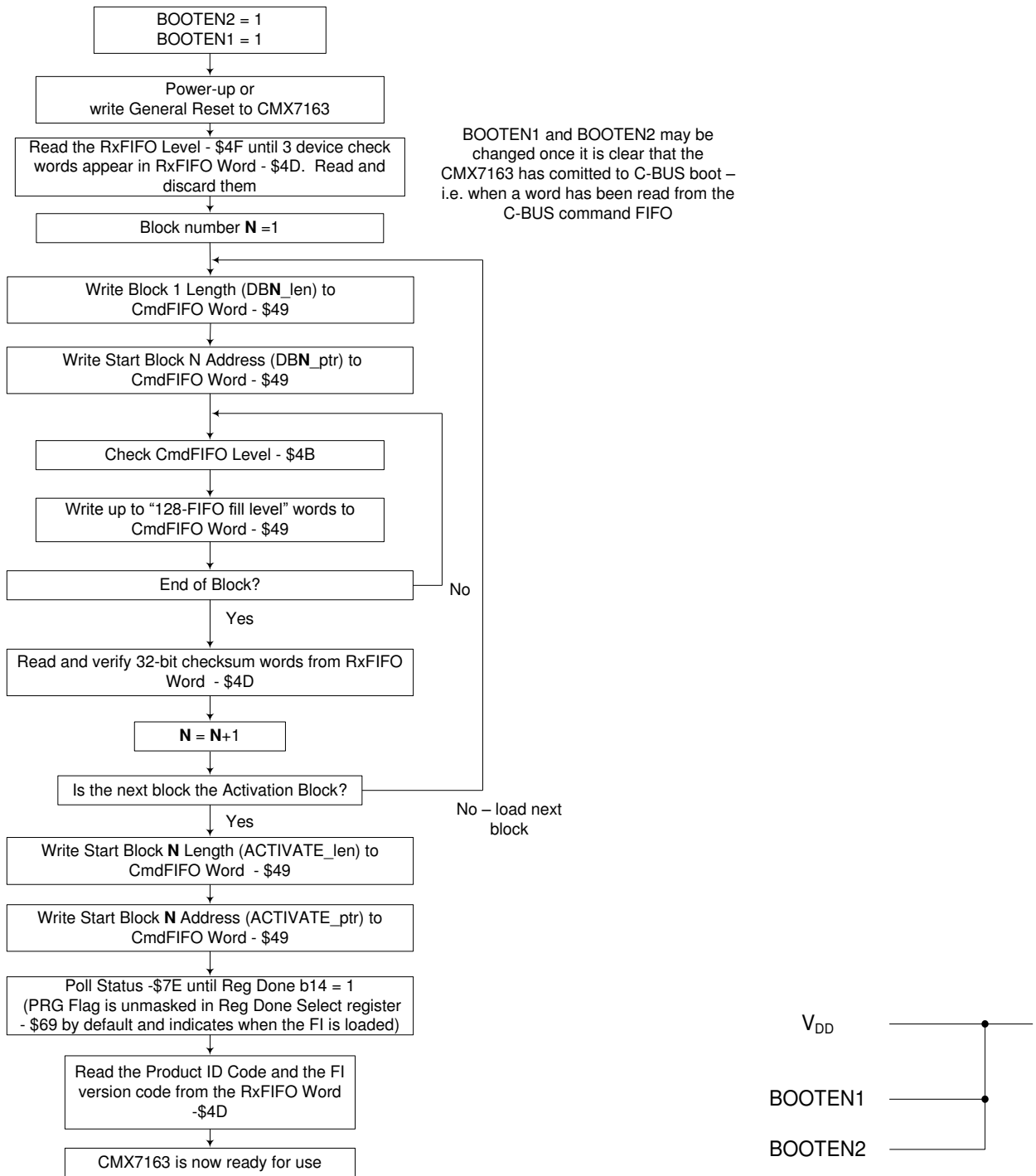
Figure 8 FI Loading from Host
