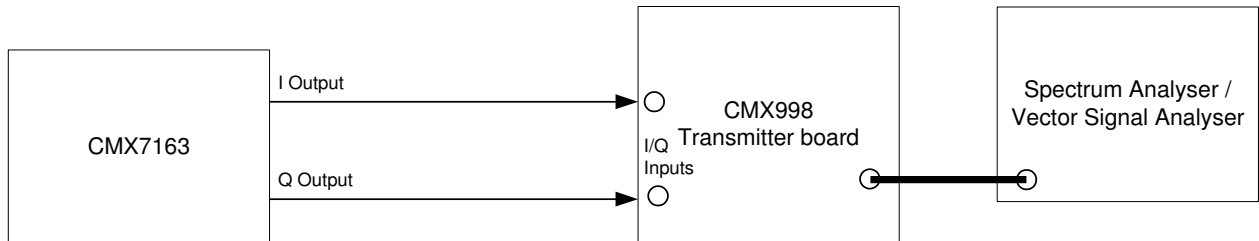
Figure 33 Tx Spectrum and Modulation Measurement Configuration for I/Q Operation
