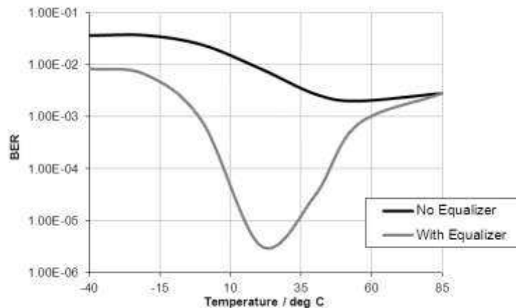
Figure 50 Performance of 64-QAM equalised signals with temperature variation
