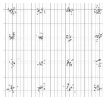
Figure 22 Normalised Constellation (noisy received signal)
