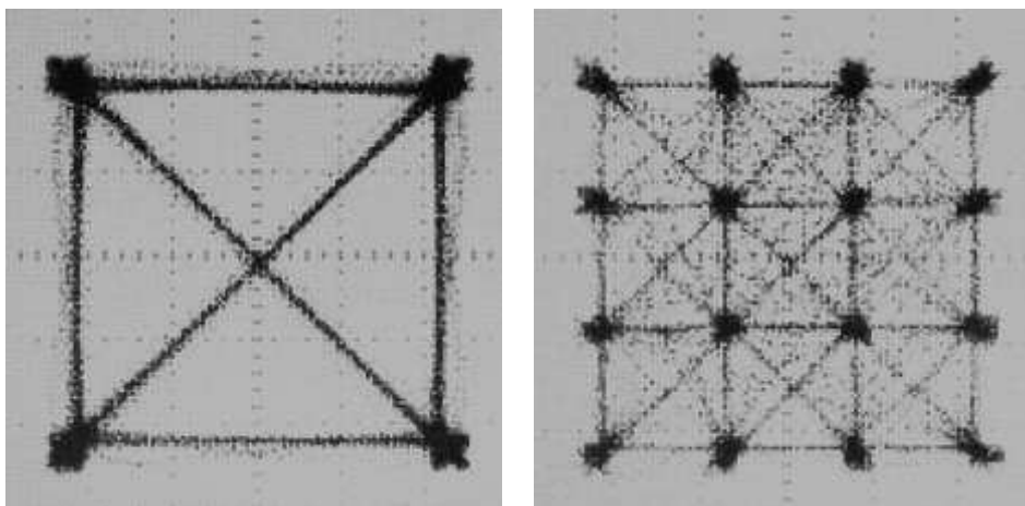
Figure 32 Received 4 and 16-QAM signals with equalisation
