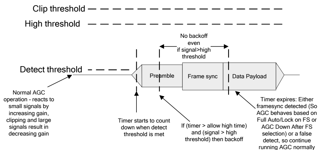
Figure 25 AGC Behaviour During Burst Reception
