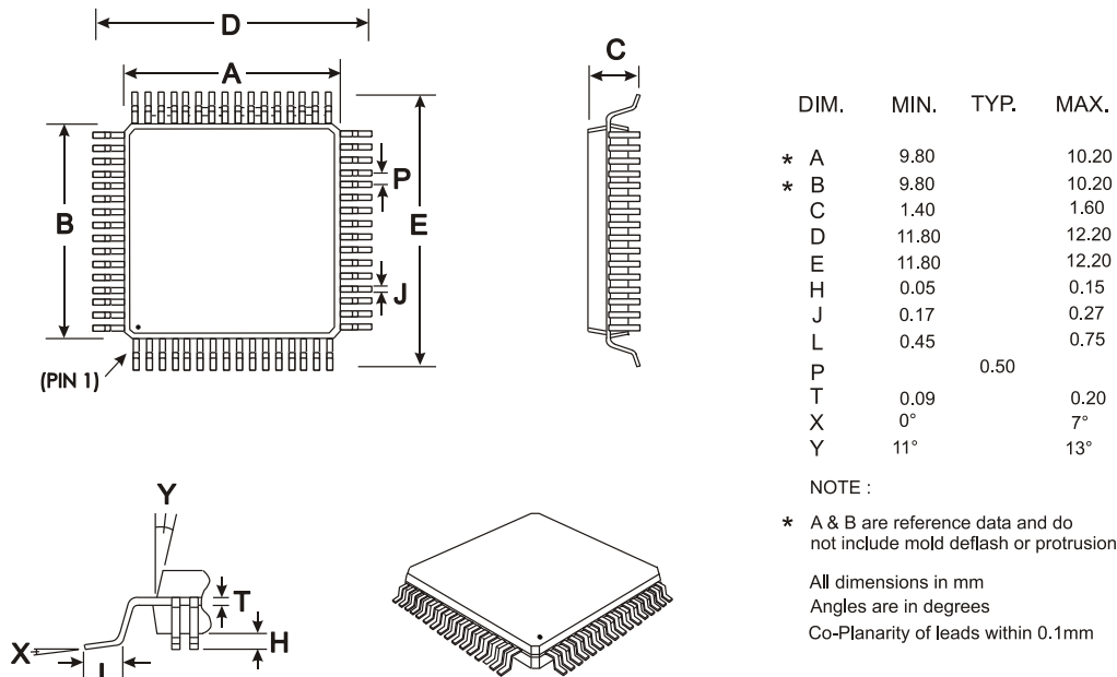
Figure 52 Mechanical Outline of 64-pin LQFP (L9)
