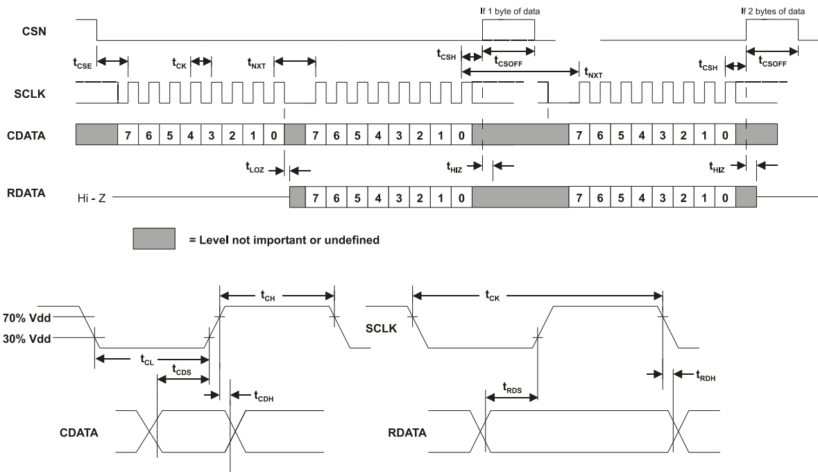
Figure 53 C-BUS Timing
