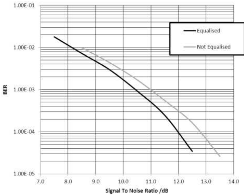
Figure 46 4-QAM Signal to Noise Performance, Equalised and Not Equalised
