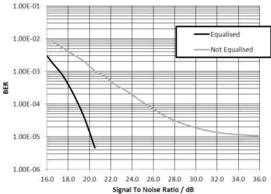
Figure 47 16-QAM Signal to Noise Performance, Equalised and Not Equalised
