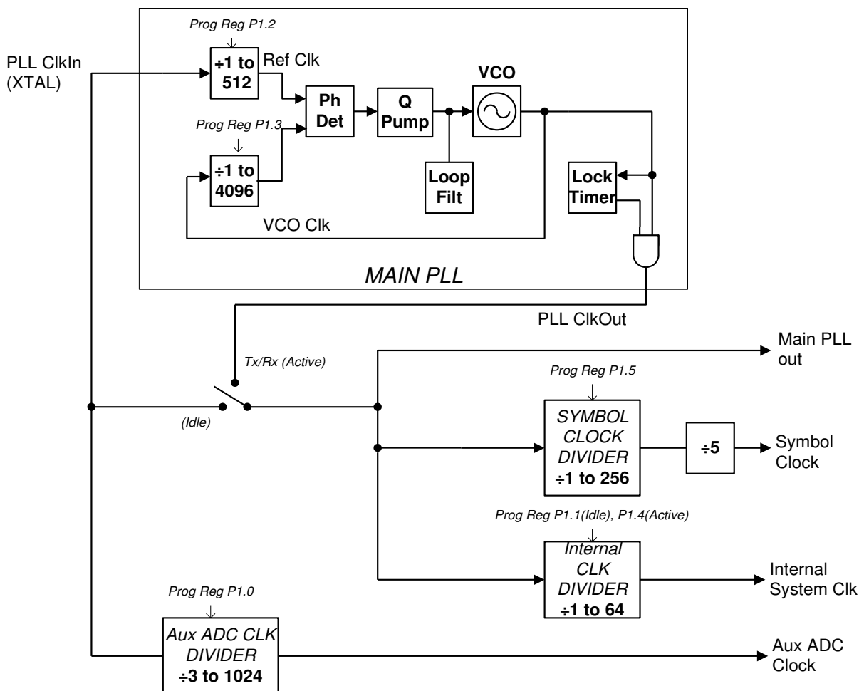
Figure 26 Main Clock Generation
