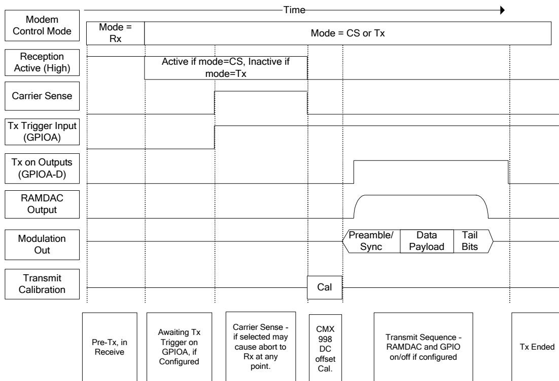
Figure 13 Transmit Sequence
