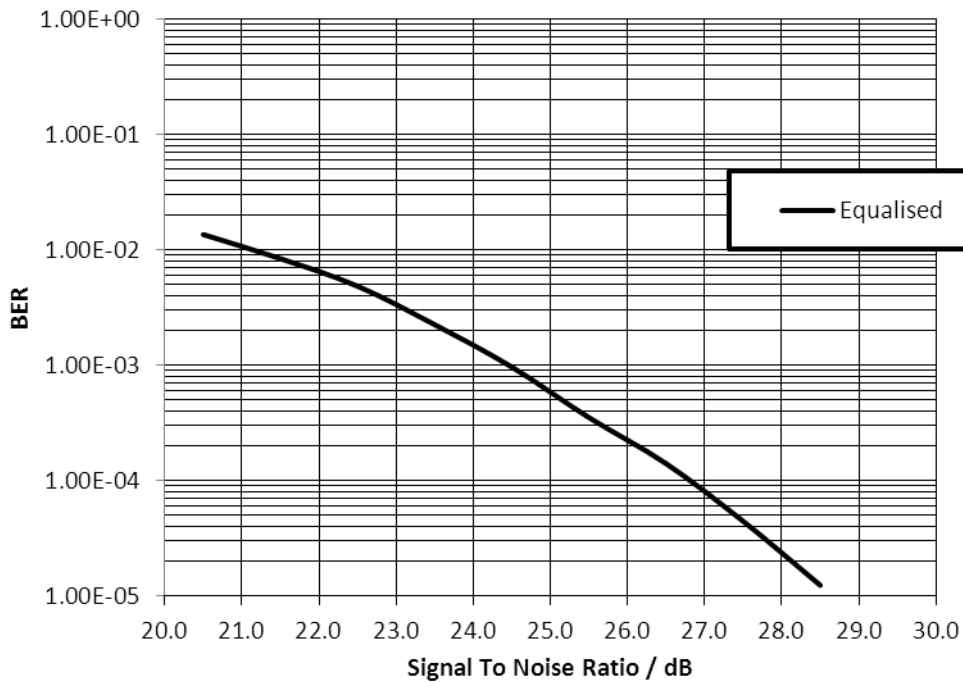
Figure 48 64-QAM Signal to Noise Performance, Equalised
