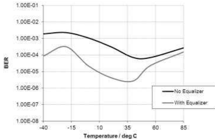
Figure 49 Performance of 16-QAM equalised signals with temperature variation
