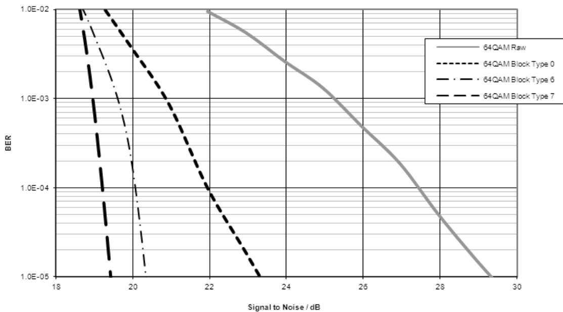
Figure 42 64-QAM Performance with Different Coding Schemes
