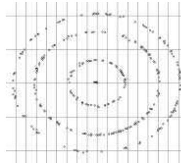
Figure 20 Sample at symbol timing with I/Q dc offset diagnostic mode (with frequency error)
