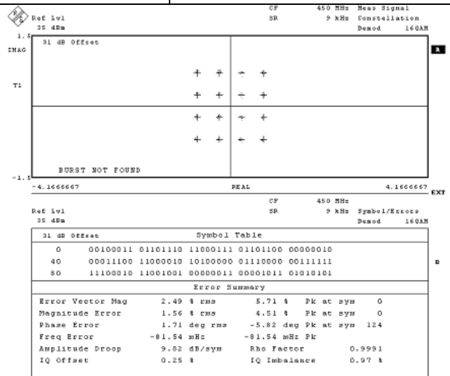
Error Vector
