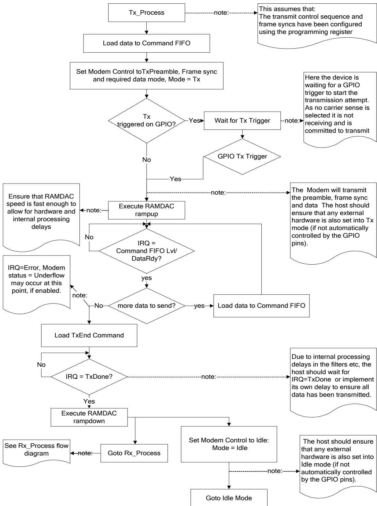
Figure 10 Host Tx Data Flow (No Tx Sequence/Carrier Sense)
