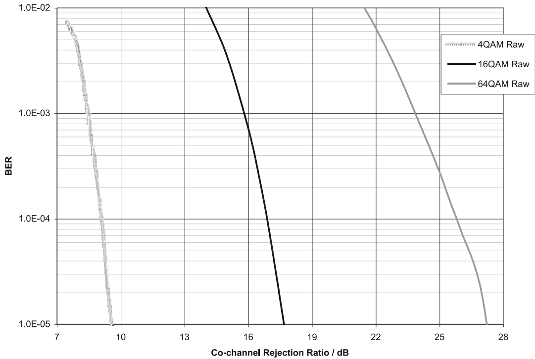
Figure 39 Modem Co-Channel Rejection with FM Interferer (as EN 300 113)
