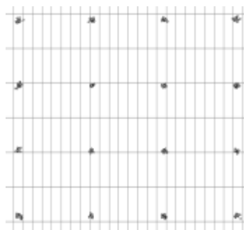
Figure 21 Normalised Constellation (even with a frequency or phase error)
