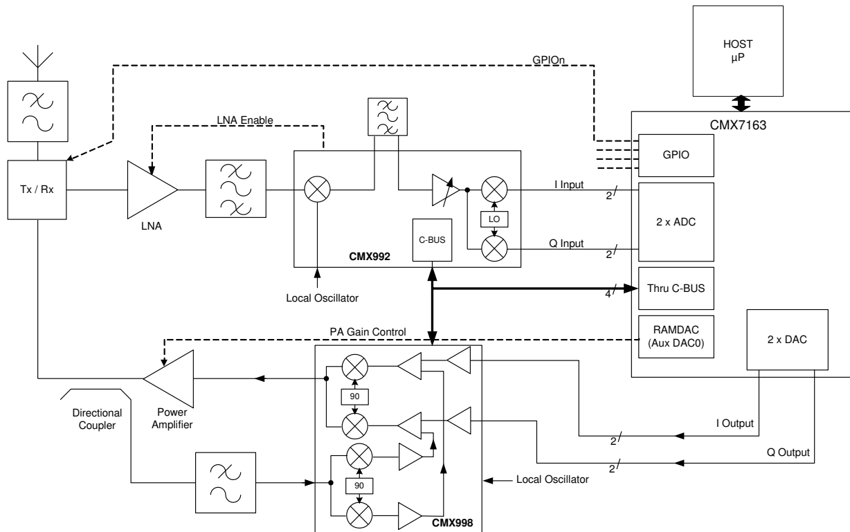
Figure 29 Outline Radio Design (I/Q in/out for QAM)
