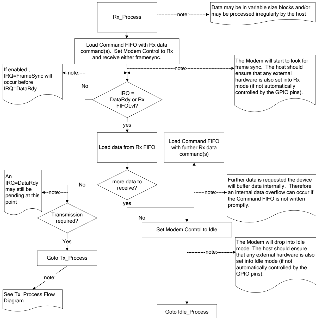
Figure 11 Host Rx Data Flow
