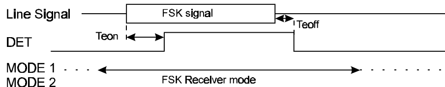
Figure 4 : FSK Level Detector operation
