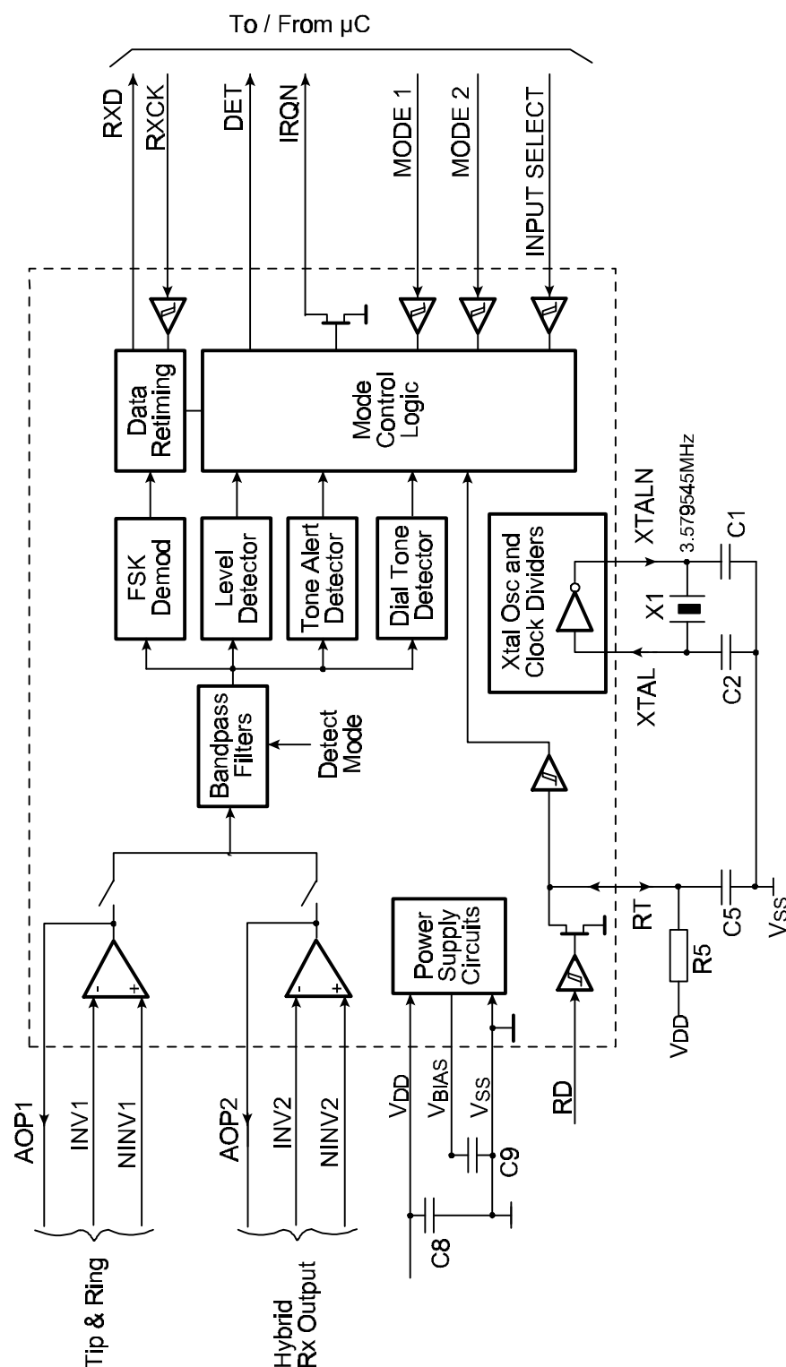
Figure 1 : Block Diagram
