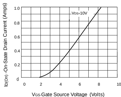
Transfer Characteristics
