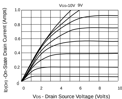
Saturation Characteristics
