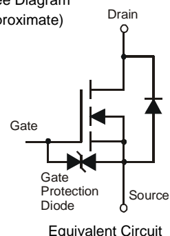
Equivalent Circuit
