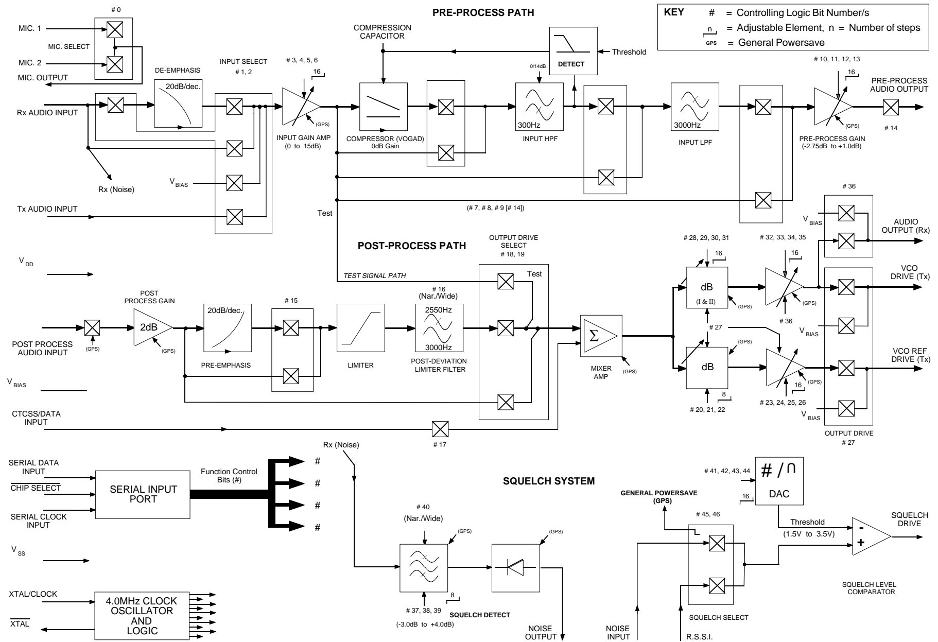
Fig.4 PMR Audio Processor – Facilities
