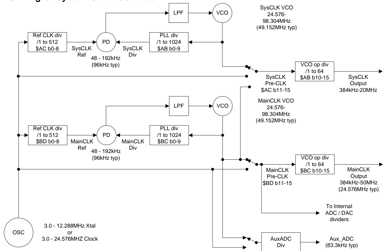
Figure 15 Digital Clock Generation Schemes
