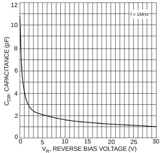
Fig. 4 Output Capacitance
