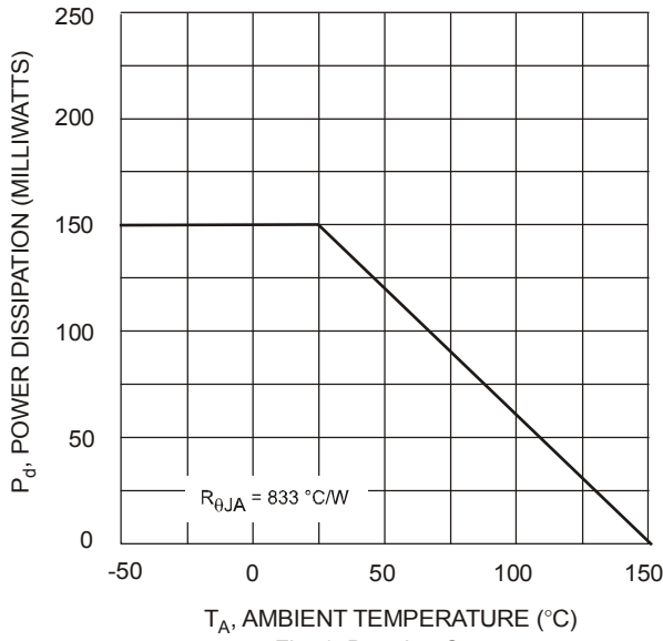
Fig. 1 Derating Curve
