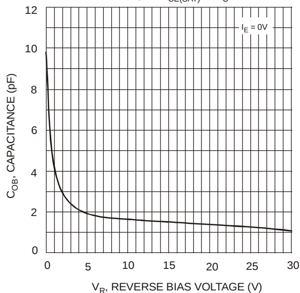
Fig. 4 Output Capacitance
