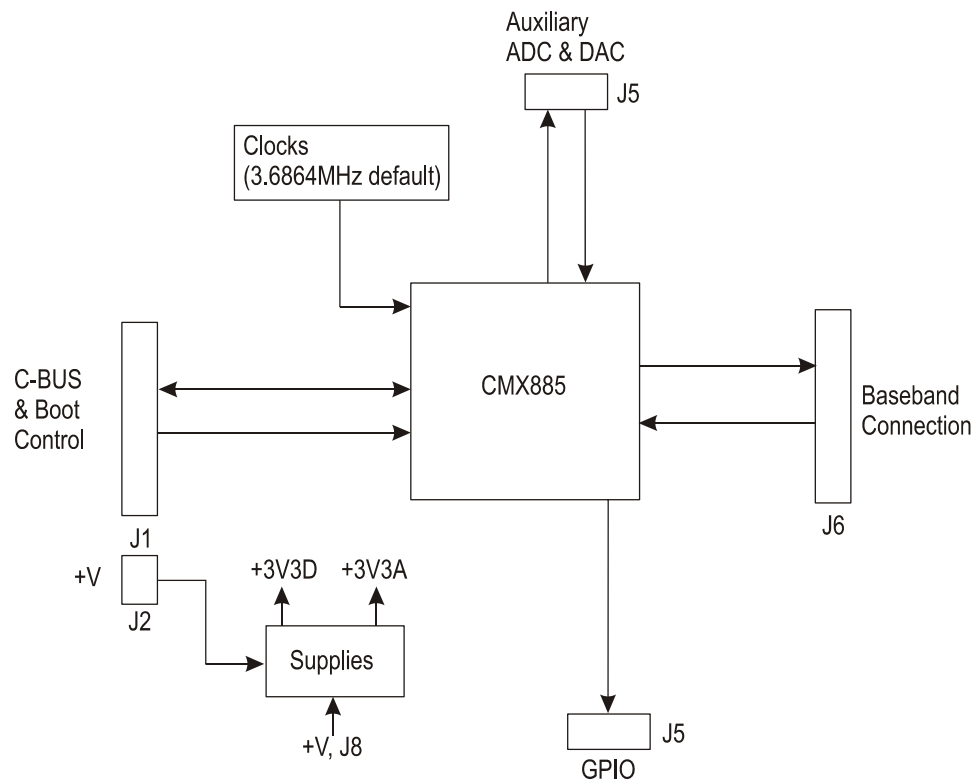
Figure 1 – Block Diagram
