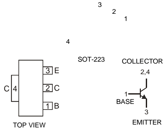
Schematic and Pin Configuration
