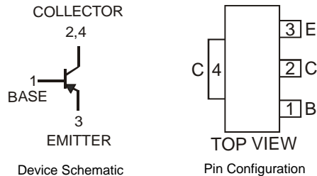
Device Schematic
