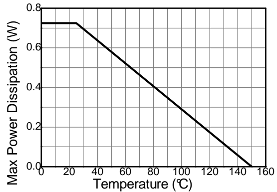
Derating Curve
