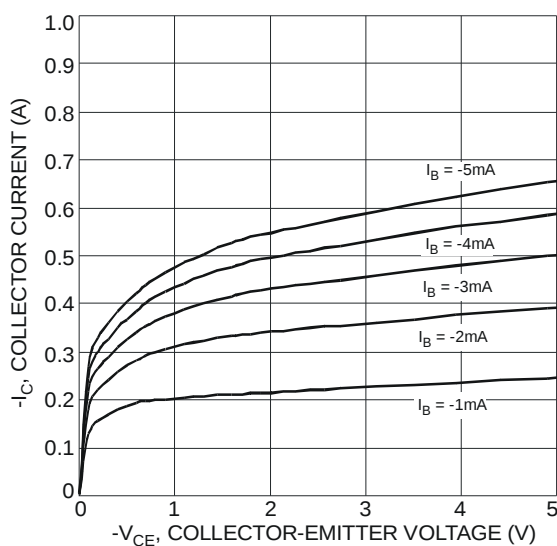
Fig. 4 Typical Collector Current vs. Collector-Emitter Voltage
