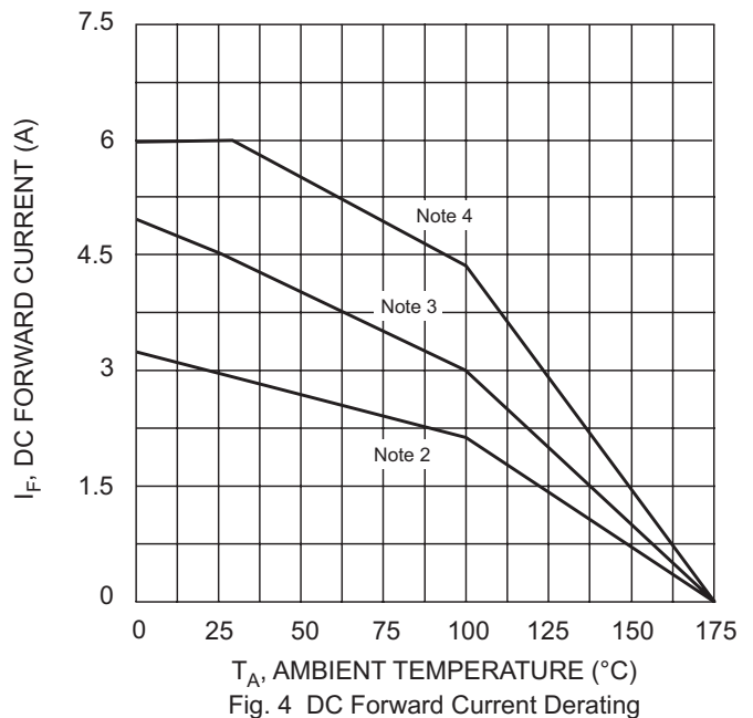
Fig. 4 DC Forward Current Derating
