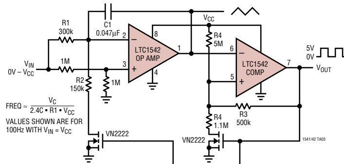
Voltage Control Oscillator
