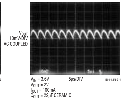
Output Ripple, C_{OUT} = 22\mu\text{F}
