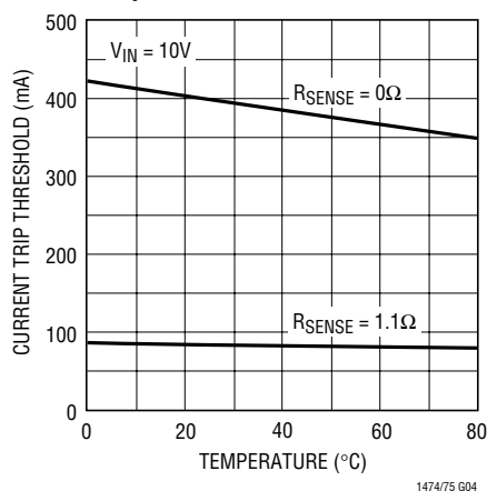
Current Trip Threshold vs Temperature
