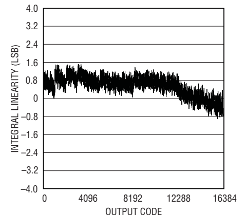
Integral Linearity End Point Fit for CH1 with Internal 2.5V Reference for Differential Input Signals
