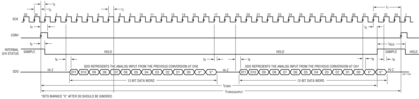
LTC1407-1 Timing Diagram
