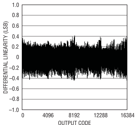
Differential Linearity for CH1 with Internal 2.5V Reference
