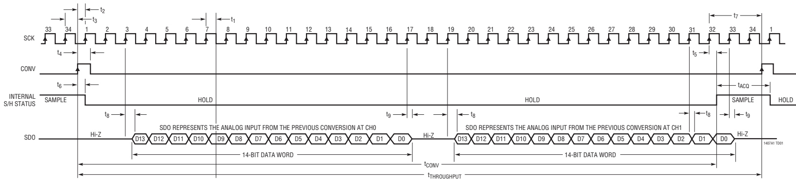
LTC1407A-1 Timing Diagram
