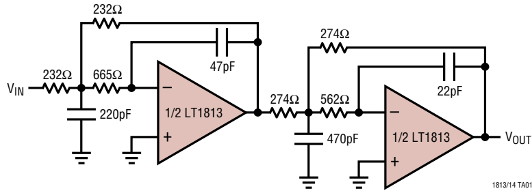
4MHz, 4th Order Butterworth Filter
