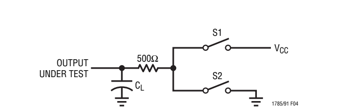
Figure 4. Driver Timing Test Load
