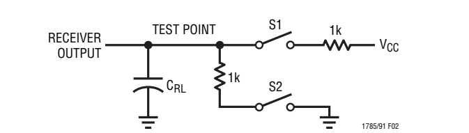
Figure 2. Receiver Timing Test Load
