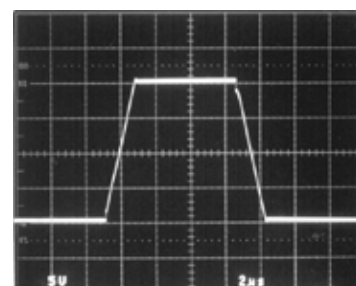
±15V Large-Signal Response
