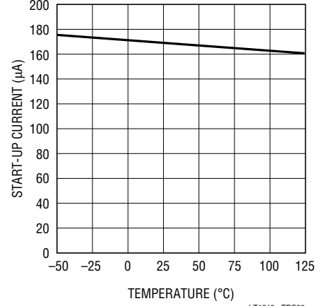
Start-Up Current
