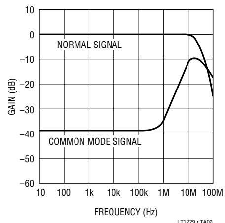
Loop Through Amplifier Frequency Response
