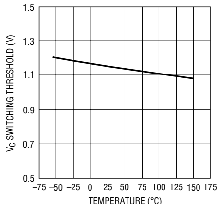
V C Switching Threshold Voltage vs Temperature
