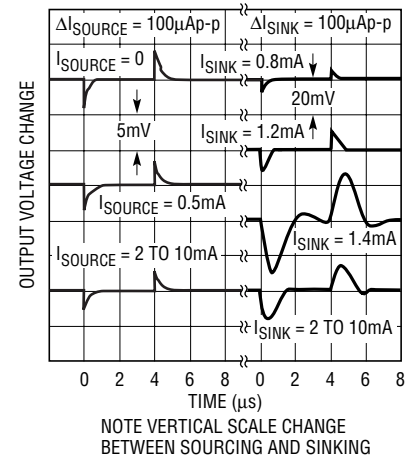
Load Transient Response C_{\text{LOAD}} = 1000\text{pF}
