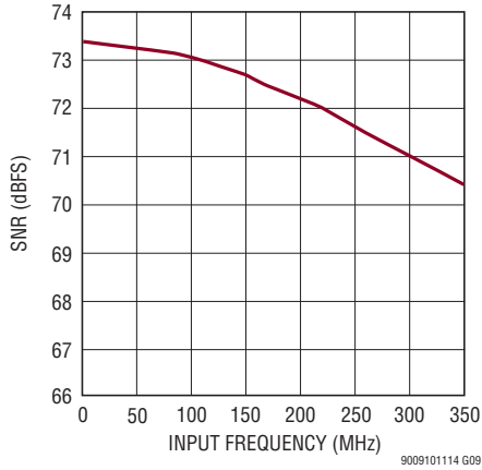
LTM9011-14: SNR vs Input Frequency, -1dBFS, 2V Range, 125Mps
