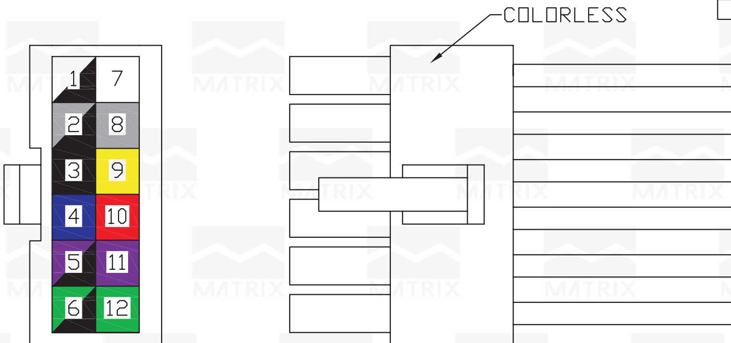
BACK SIGHT (SEEN OF THE WIRE)
