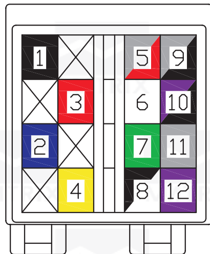
BACK SIGHT (SEEN OF THE WIRE)
