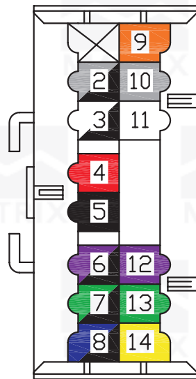
BACK SIGHT (SEEN OF THE WIRE)
