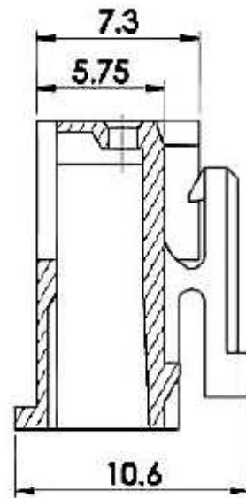
SEC. O-O'
