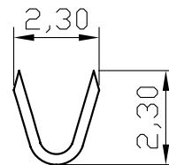
B-B SECTION
