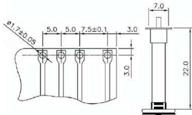
Recomand PCB Layout And Assembly Layout
