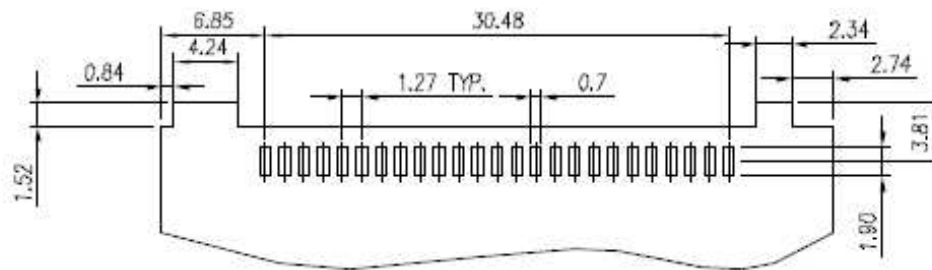
RECOMMENDED P.C.B. PATTERN
