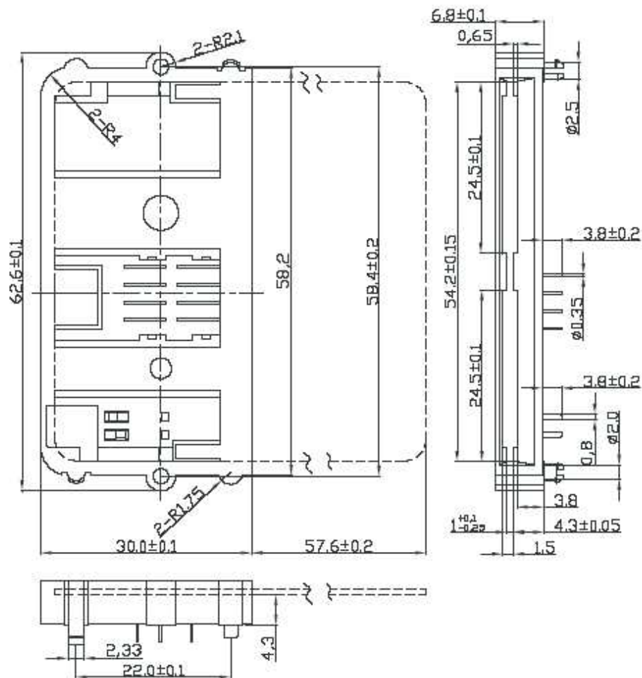
Unit: mm; Tolerances: \pm 0.15 mm Reference dimension for PCB layout
