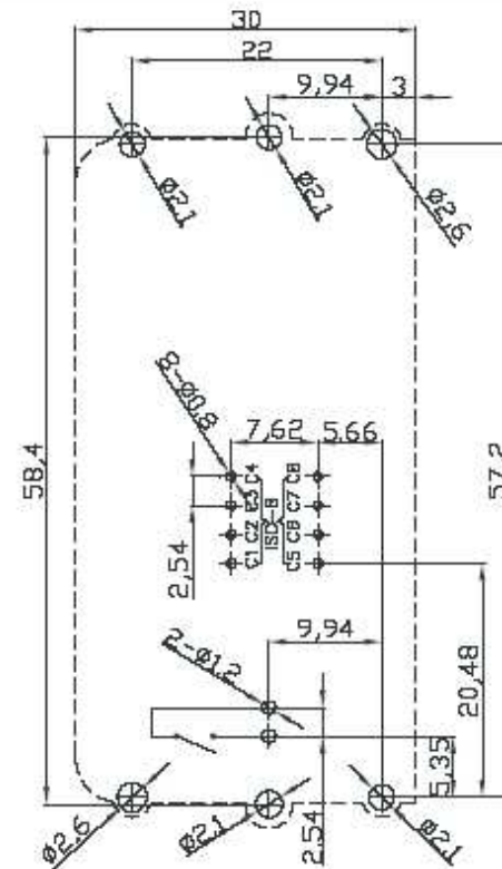
Unit: mm; Tolerances: \pm 0.15 mm Reference dimension for PCB layout
