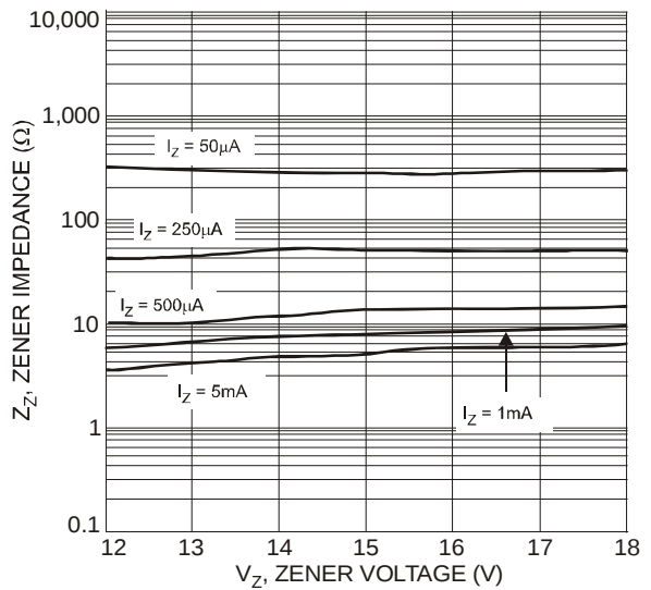
Fig. 13 Typical Zener Impedance Characteristics, DDZ9699S - DDZ9705S
