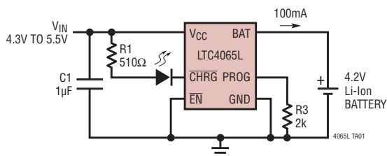
Standalone Li-Ion Battery Charger
