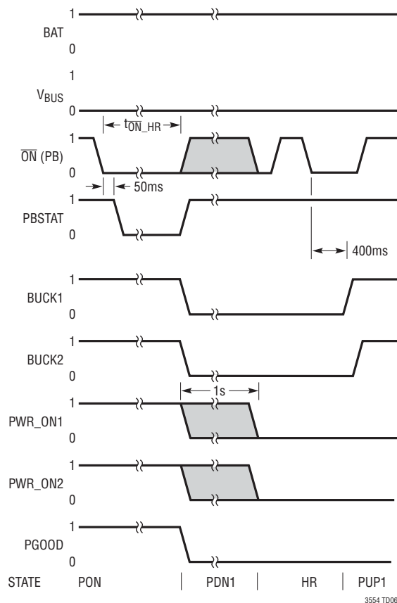
Figure 12. Hard Reset Via Holding \overline{\text{ON}} Low
