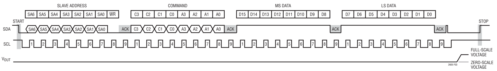
Figure 3. Typical LTC2605 Input Waveform—Programming DAC Output for Full-Scale
