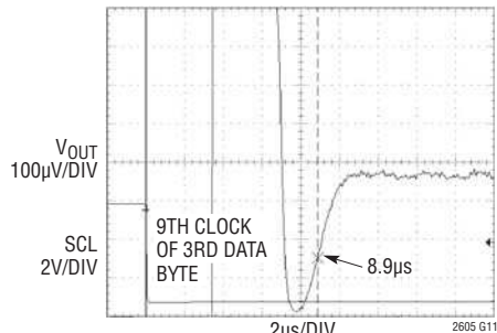
Settling to \pm 1LSB
