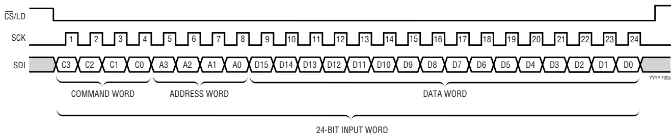
Figure 2a. LTC2602 24-Bit Load Sequence (Minimum Input Word) LTC2612 SDI Data Word 14-Bit Input Code + 2 Don't Care Bits LTC2622 SDI Data Word 12-Bit Input Code + 4 Don't Care Bits
