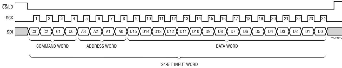
Figure 2a. LTC2600 24-Bit Load Sequence (Minimum Input Word). LTC2610 SDI Data Word: 14-Bit Input Code + 2 Don't-Care Bits; LTC2620 SDI Data Word: 12-Bit Input Code + 4 Don't-Care Bits
