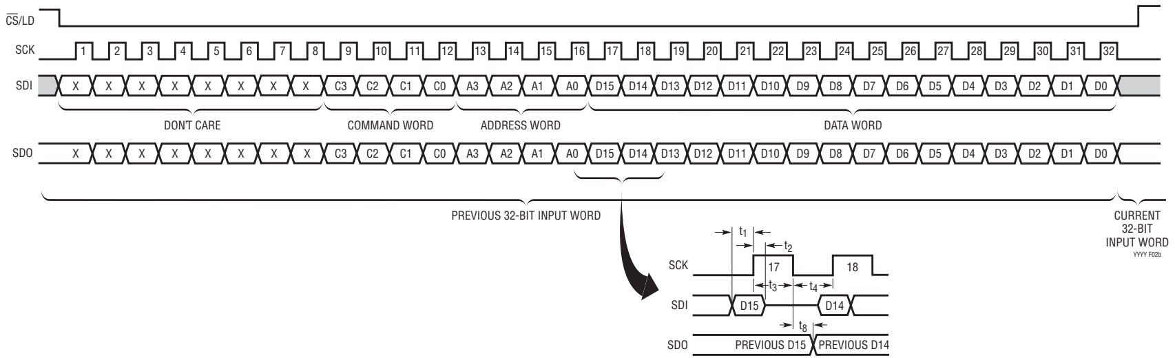
Figure 2b. LTC2600 32-Bit Load Sequence (Required for Daisy-Chain Operation). LTC2610 SDI/SDO Data Word: 14-Bit Input Code + 2 Don't-Care Bits; LTC2620 SDI/SDO Data Word: 12-Bit Input Code + 4 Don't-Care Bits
