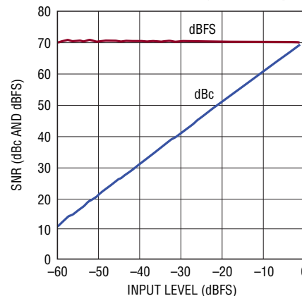
LTC2268-12: SNR vs Input Level, f_{IN} = 70\text{MHz} , 2V Range, 125Mps
