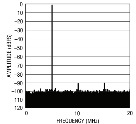
LTC2264-12: 8k Point FFT, f_{IN} = 5\text{MHz} , -1dBFS, 40Msps
