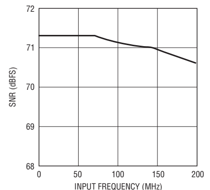
LTC2228: SNR vs Input Frequency, -1dB, 2V Range, 65Mpsps
