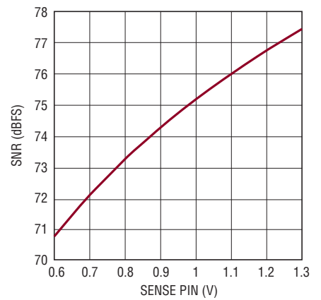
LTC2190: SNR vs SENSE, f_{IN} = 5\text{MHz} , -1\text{dBFS}
