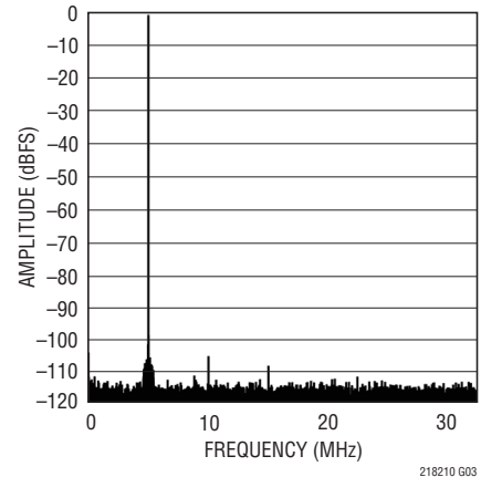
LTC2182: 64k Point FFT, f_{IN} = 5\text{MHz} , -1dBFS, 65Msps
