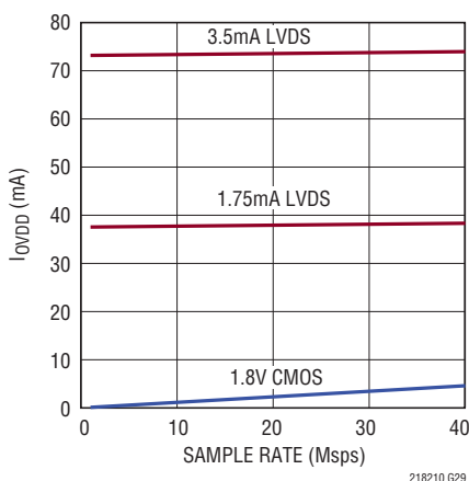
LTC2181: I_{OVPD} vs Sample Rate, 5MHz, -1dBFS, Sine Wave Input on Each Channel
