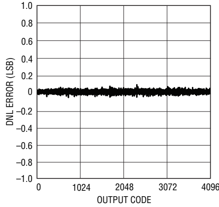
LTC2172-12: Differential Nonlinearity (DNL)
