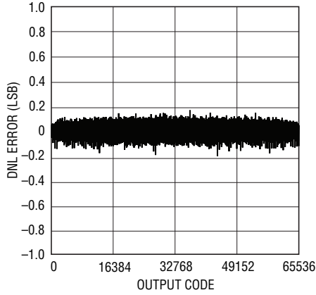
LTC2165 Differential Non-Linearity (DNL)
