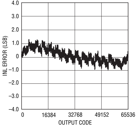
LTC2165 Integral Non-Linearity (INL)
