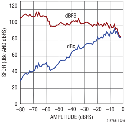
LTC2155-14: SFDR vs Input Level, f_{IN} = 70\text{MHz} , 170Msps
