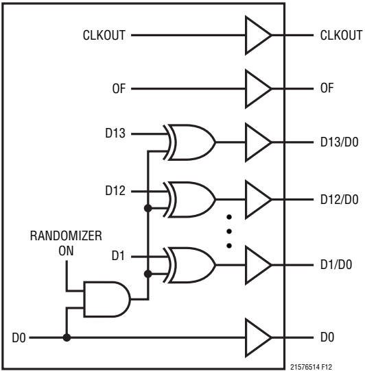
Figure 12. Functional Equivalent of Digital Output Randomizer
