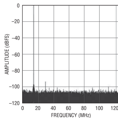
LTC2157-14 32K Point FFT, f_{\text{IN}} = 15\text{MHz} , -1\text{dBFS} , 250Msps
