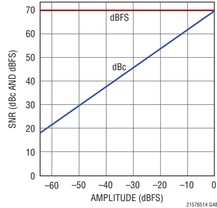
LTC2155-14: SNR vs Input Level, f_{IN} = 70\text{MHz} , 170Msps
