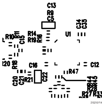
Silkscreen Top
