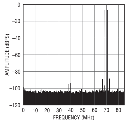
LTC2150-12: 32K Point 2-Tone FFT, f_{IN} = 71\text{MHz} and 69\text{MHz} , 170\text{Mps}
